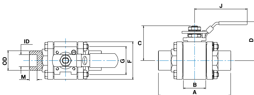
H-510 TUBE SOCKET WELD STANDARD CONFIGURATION DIMENSIONS
