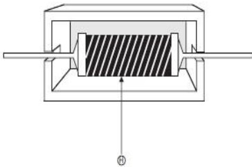
FLUTING CEMENT TYPE 刻槽水泥电阻
