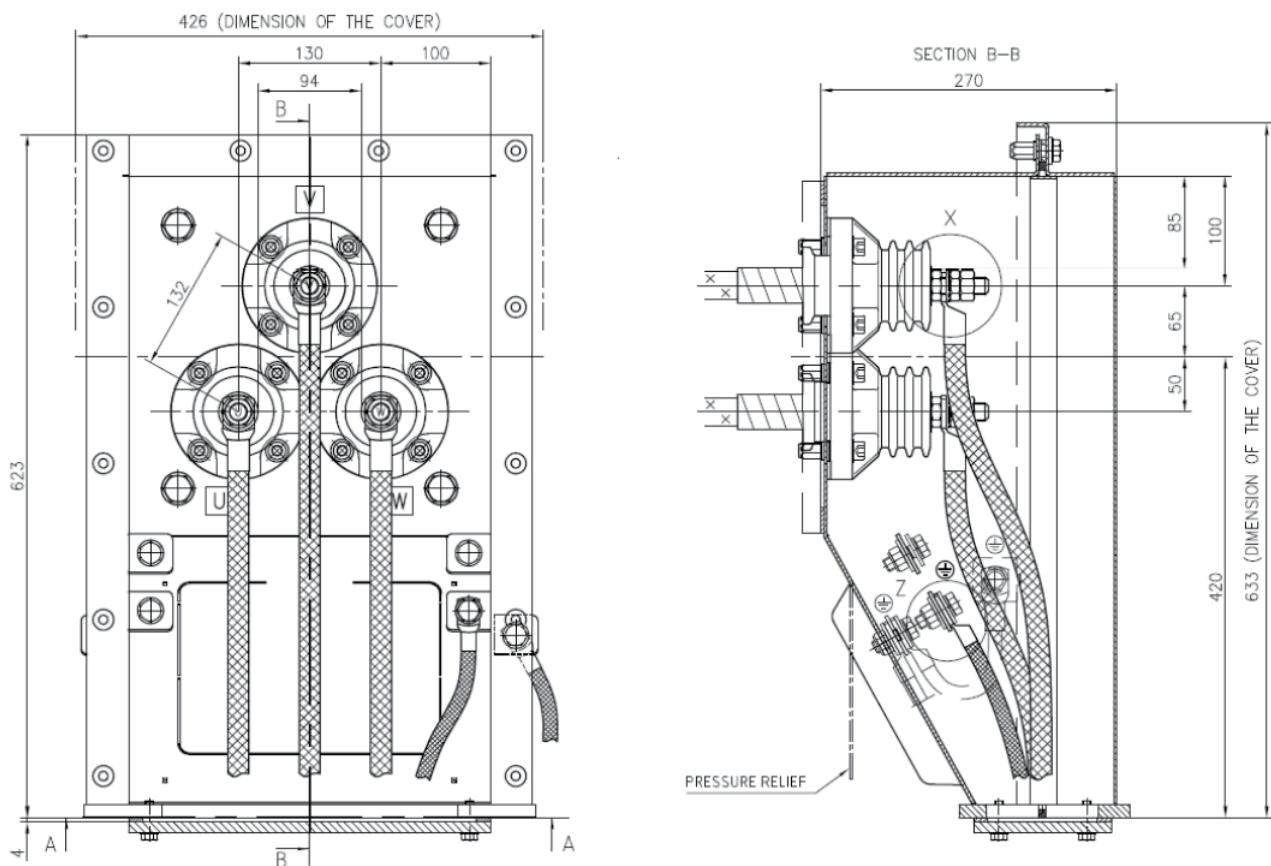
Figure above: High voltage terminal box. Dimensions in mm.
