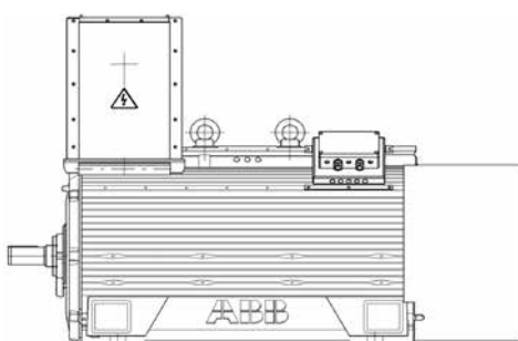
Code I: IM B3 Code II: IM 1001 Standard floor mounting, feet facing downwards (Horizontal foot mounted)
