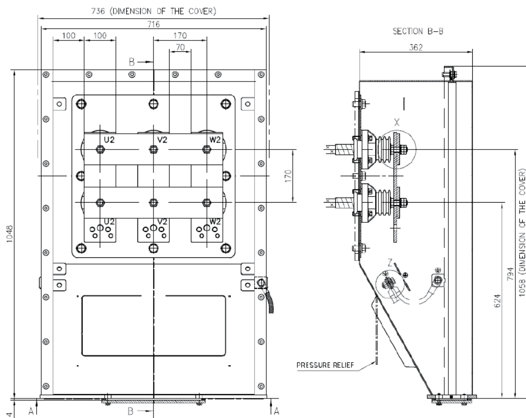
Figure above: High voltage star point terminal box, max 6.6 kV. Dimensions in mm.
