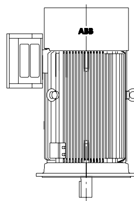
Code I: IM V1 Code II: IM 3011 Flange and free shaft end facing downwards (Vertical solid shaft, flange mounted)
