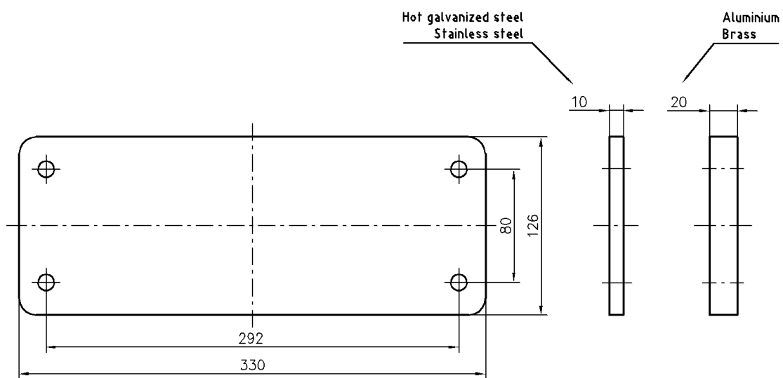
Figure above: Blind flange FL 33 for main terminal box.
