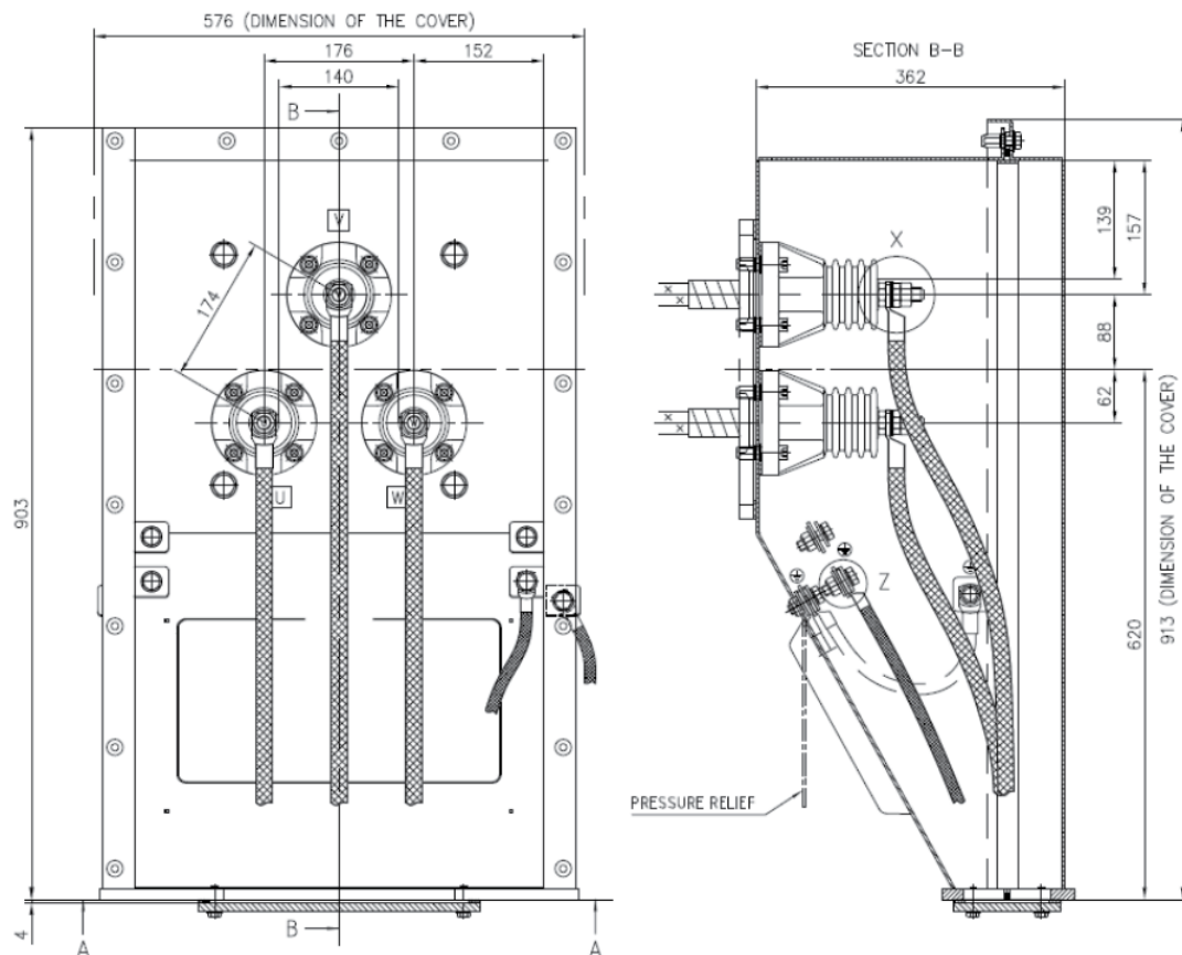
High voltage terminal box up to 11 kV.
