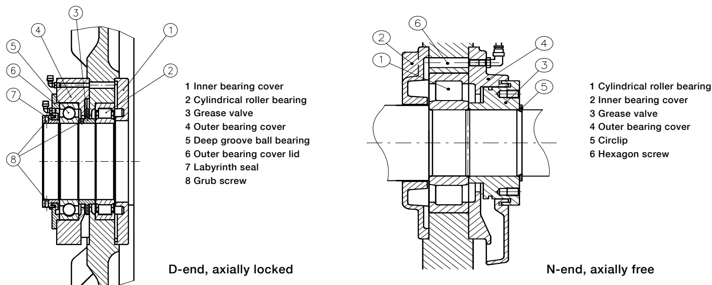
Figure: Standard bearing construction for horizontally mounted motors HXR 560.
