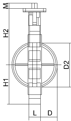
DN50 to 300
