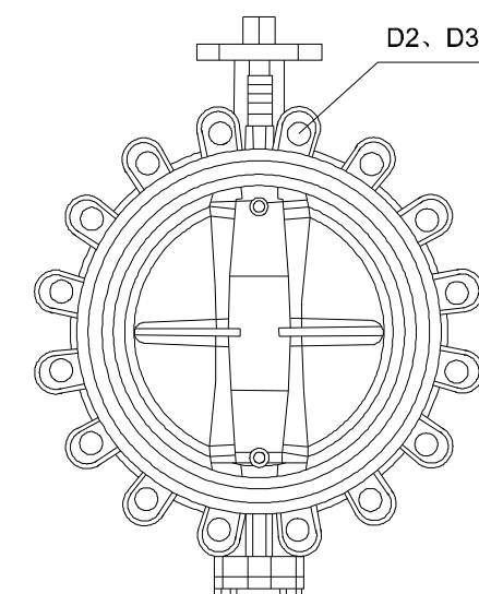
DN350 to 600
