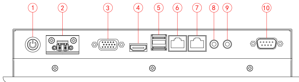
1. ON/OFF 2. DC_IN 3. VGA 4. HDMI 5. USB 6. LAN1 7. LAN2 8. MIC_IN 9. LINE_OUT 10. COM
