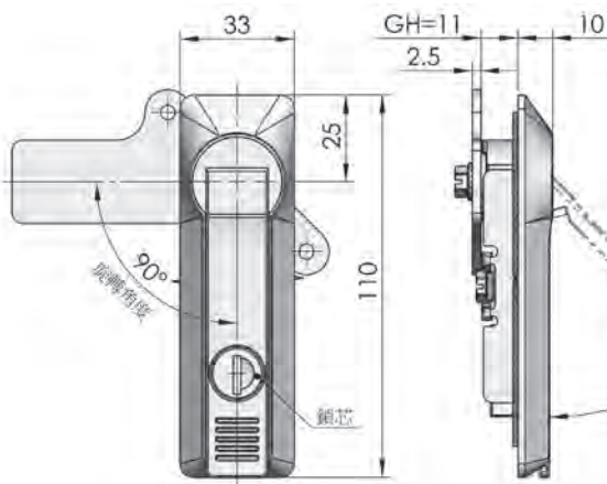
MS-723-2 (附鎖芯 Locking)
