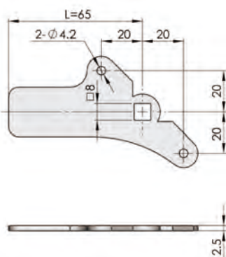
檔片 CAM
