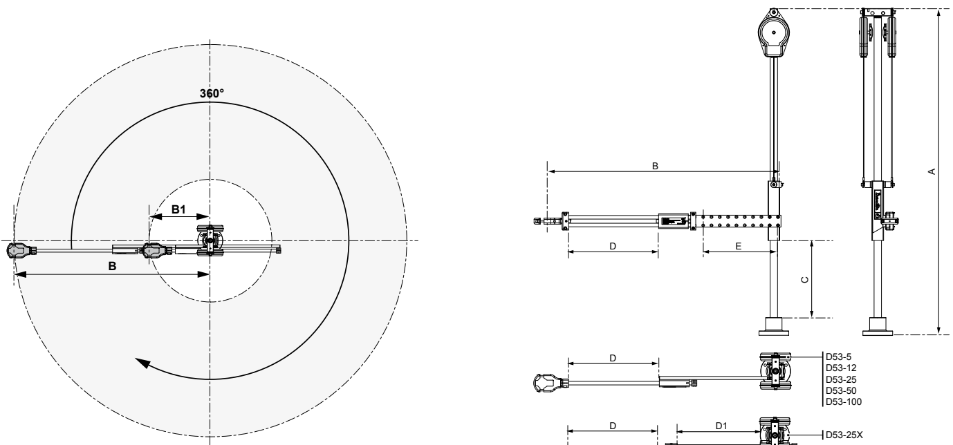
D53 linear working area product specification
