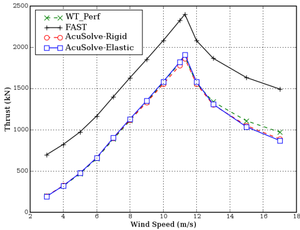
Rotor Thrust
