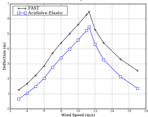
Out of Plane Tip Deflection
