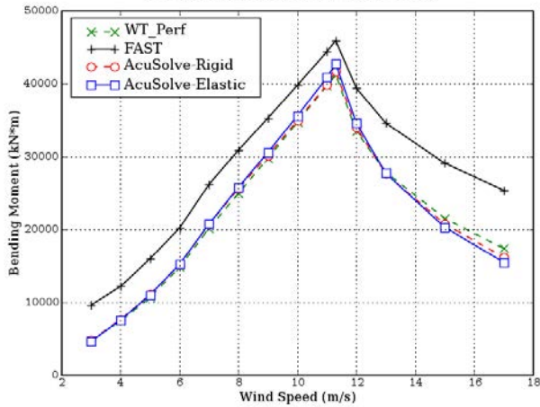
Flapwise Bending Moment
