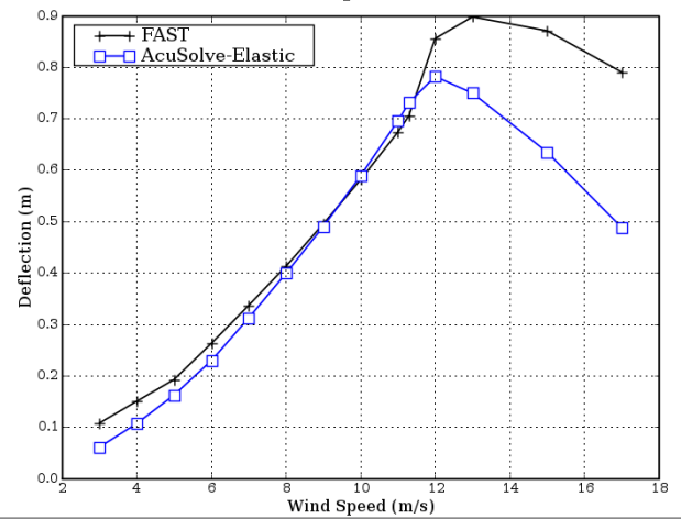
In Plane Tip Deflection
