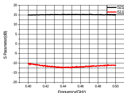
Receiver Small Signal Parameters
