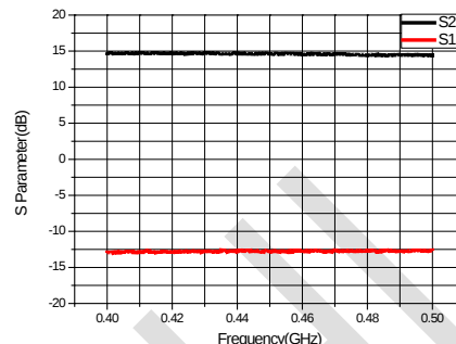
Transmitter Small Signal Parameters
