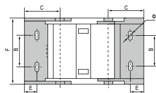
X 2 型接头 X 2 type bracket
