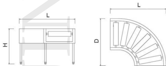
90度转角器 90 Degree Angling Equipment
