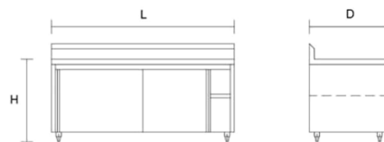
打荷台柜 / Load Cabinet
