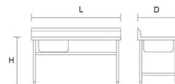
单星盆理鱼台 Single Star Basin Fish Processing Platform
