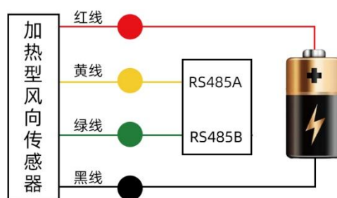
(RS485单路供电)
