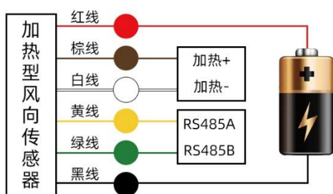
(RS485双路供电)
