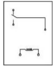
接线图(底视图) Wiring Diagram (Bottom view)
