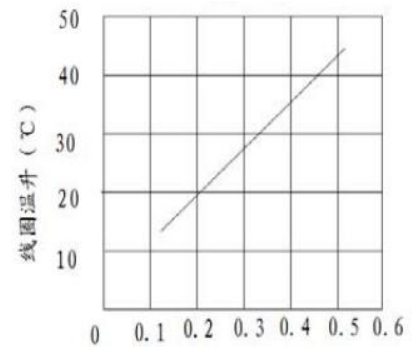
线圈功耗 Coil power consrmption(W)
