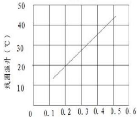
触点电流 Contact current(A)
