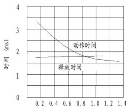
线圈功耗 Coil power consrmption(W)
