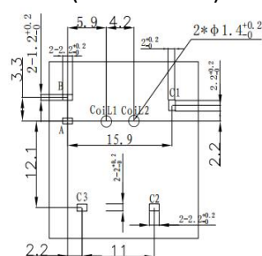
接线图(底视图) Wiring Diagram (Bottom view)
