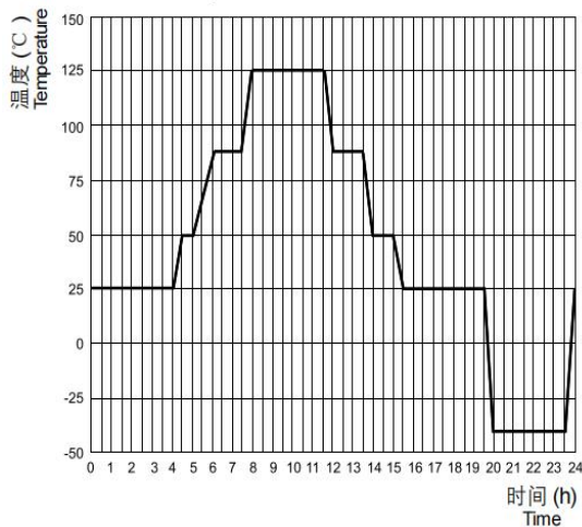
3. 电耐久试验环境温度曲线 Ambient Temperature Curve of the Electrical Endurance Test
