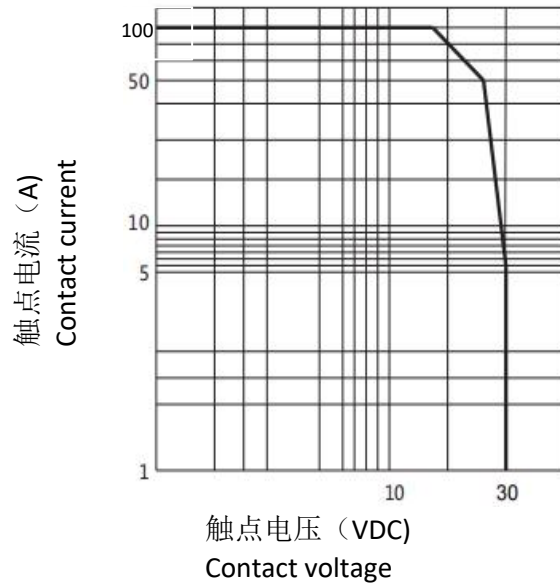
2. 允许最大负载范围 Allowable maximum load range
