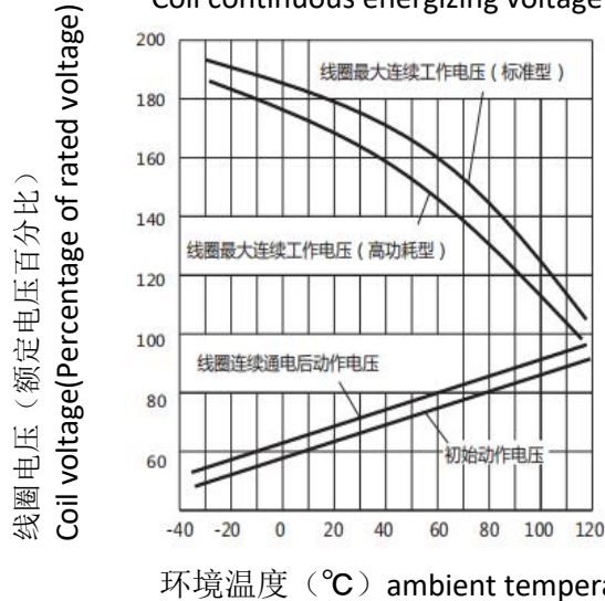
3. 电耐久试验环境温度曲线 Ambient Temperature Curve of the Electrical Endurance Test
