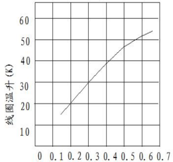
线圈温升 Coil temperature
