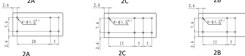
安装孔位图(底视图) PCB Layout (Bottom view)
