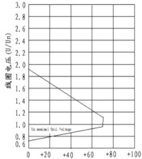
线圈温升Coil temperature
