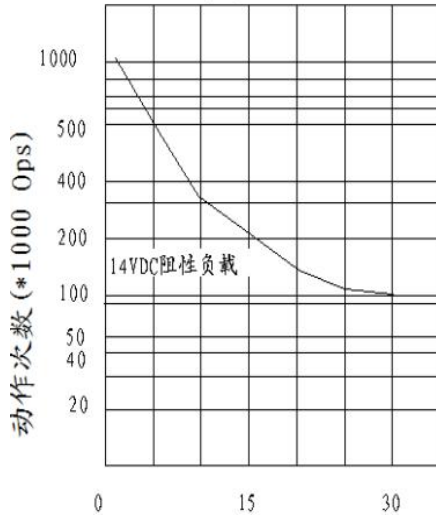
寿命曲线 Life curve
