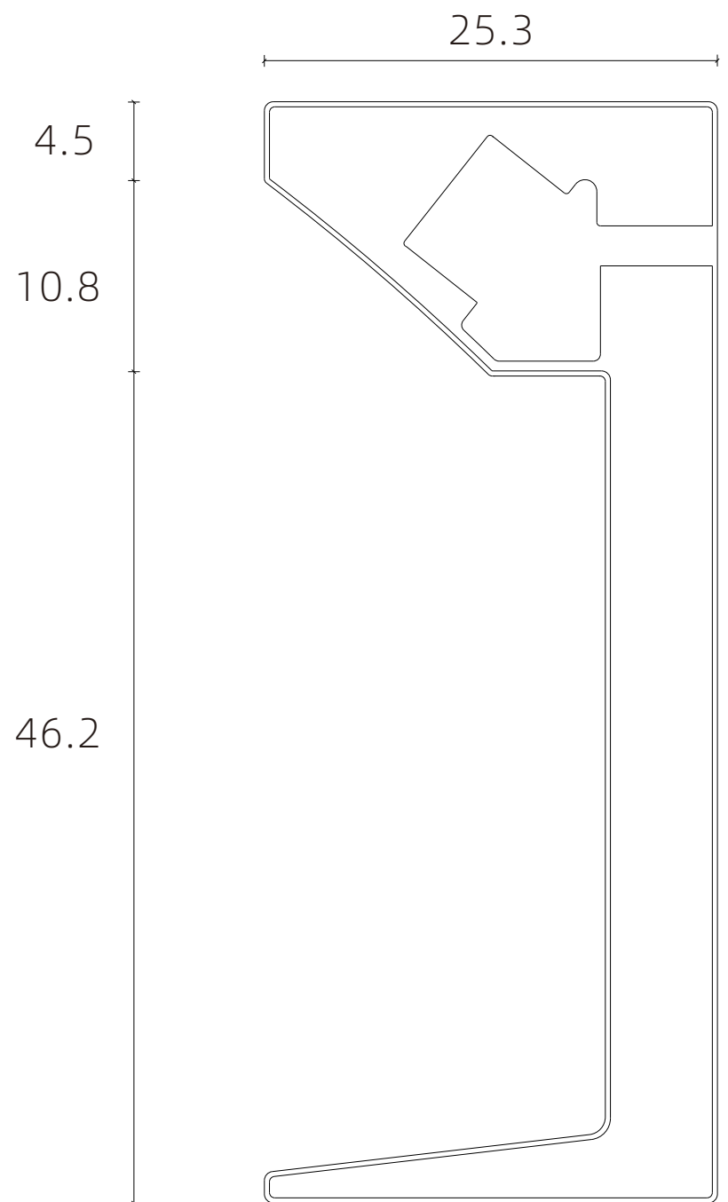
D6225锌端盖
