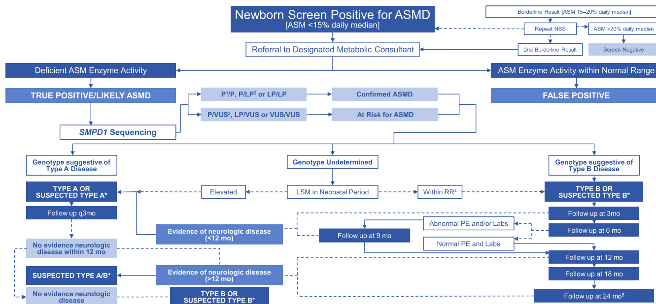
FIGURE 1 NBS algorithm.
