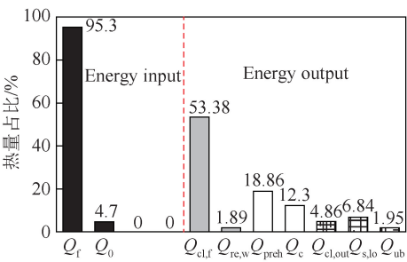
图 3 炉窑 4 个节点系统的热量收入与支出对比 Fig.3 Comparison of heat income and expense of 4 nodes system of furnace and kiln
