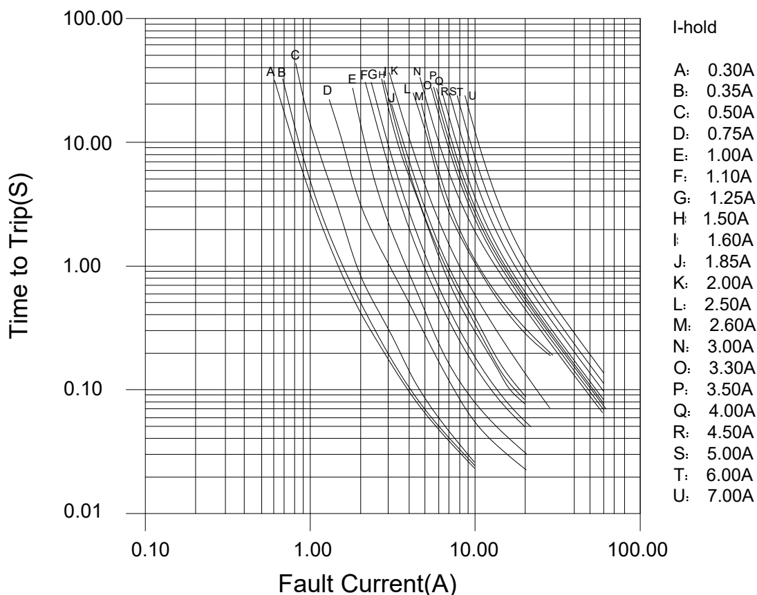
2920 Series TTT Vs Fault current chart
