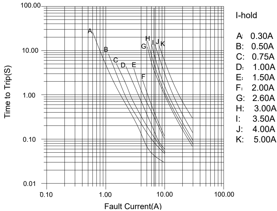
2018 Series TTT Vs Fault current chart
