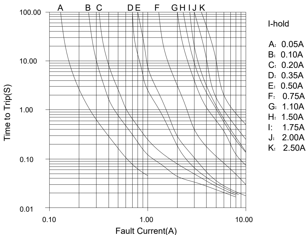
1210 Series TTT Vs Fault current chart
