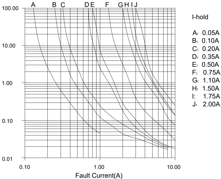
1210 Series TTT Vs Fault current chart
