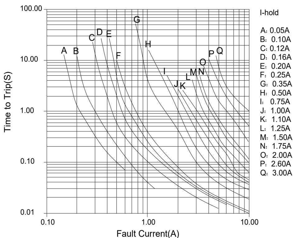
1206 Series TTT Vs Fault current chart
