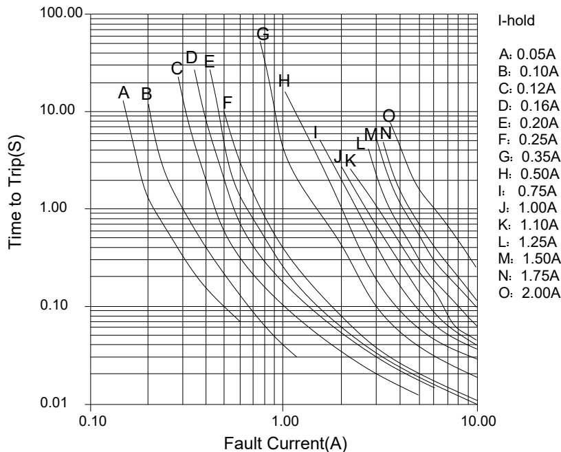
1206 Series TTT Vs Fault current chart
