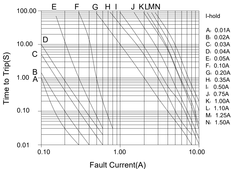
0805 Series TTT Vs Fault current chart
