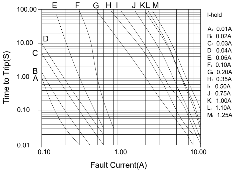
0805 Series TTT Vs Fault current chart
