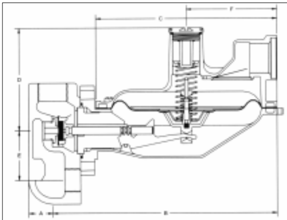
Model 1813B2-Offset
