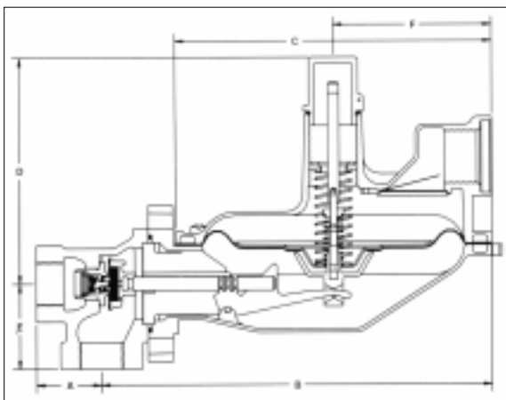
Model 1833B2-90°
