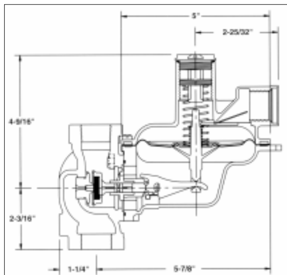
Model 1803B2-180°
