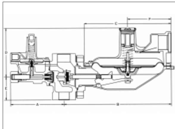
Model 1843B2
