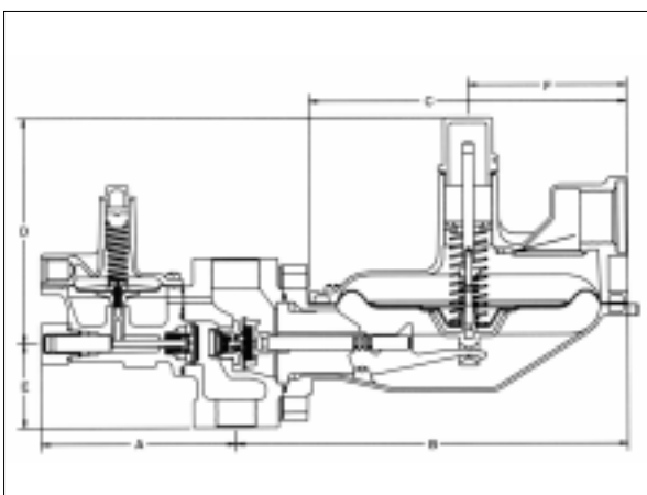
Model 1853B2
