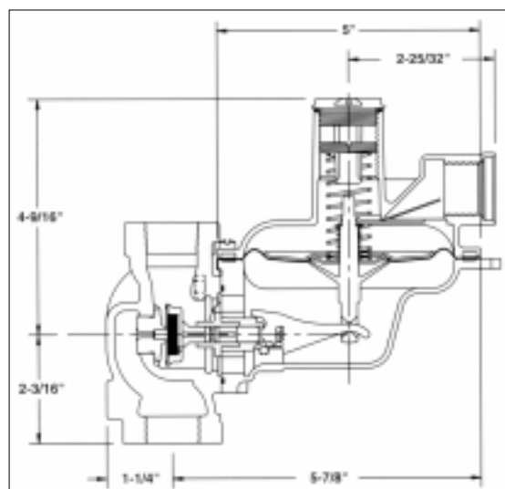
Model 1813B2-180°
