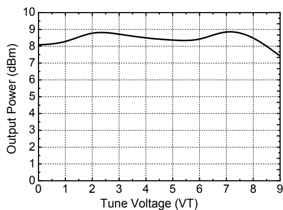
Output Power vs Tune Voltage
