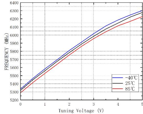
Frequency vs. Tuning Voltage vs. Temperature
