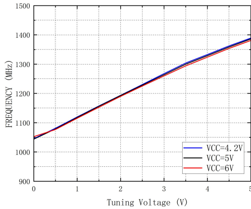
Frequency vs. Tuning Voltage vs. Operating Voltage
