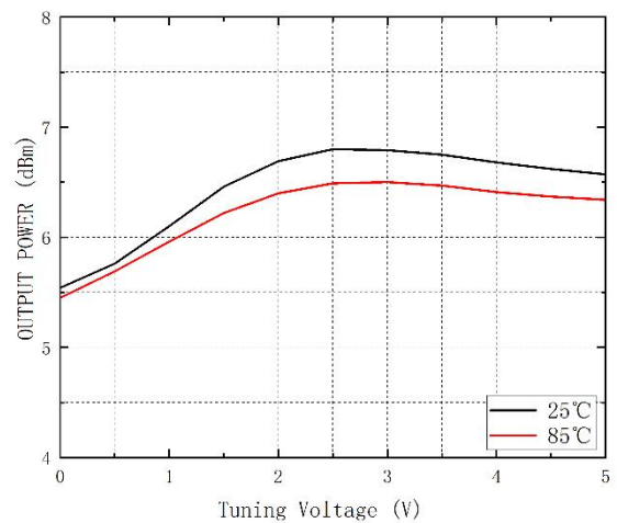
功率 vs. 调谐电压 vs. 温度@VCC=3V
