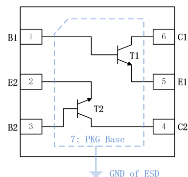
Function Block Diagram
