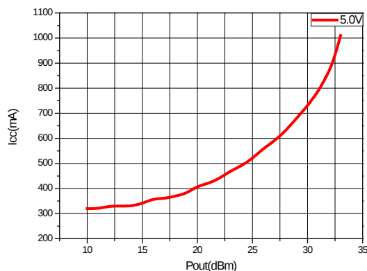
Icc vs. Output Power @2.45GHz
