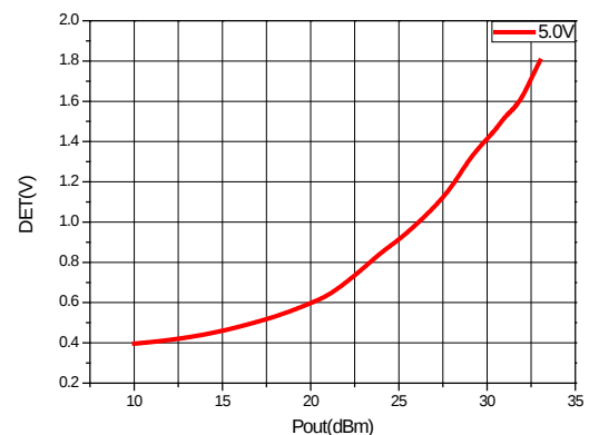
DET Voltage vs. Output Power @2.45GHz
