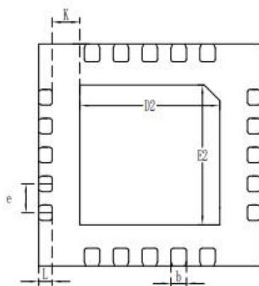
BOTTOM VIEW [底视图]
