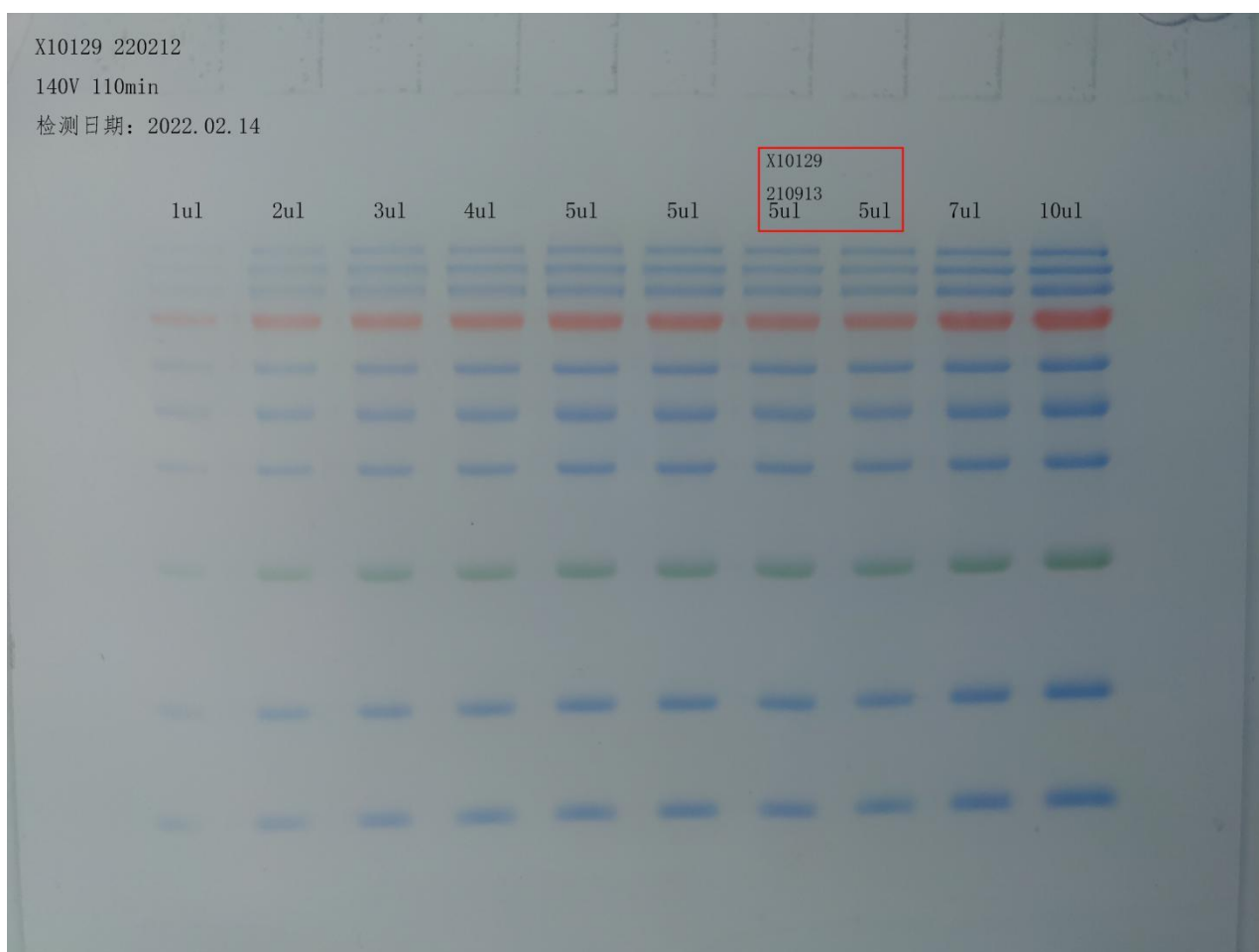
13% Tris-glycine gel (SDS-PAGE)
