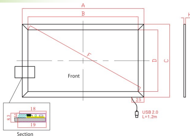
TPN-P Waterproof frame touch screen size table
