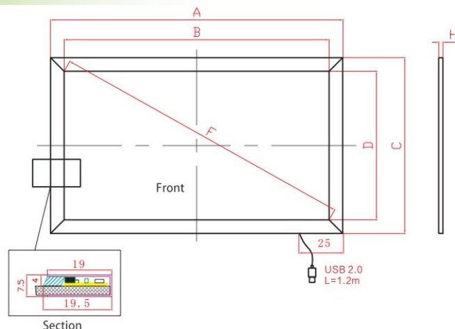
TPN-A Aluminum frame touch screen size table
