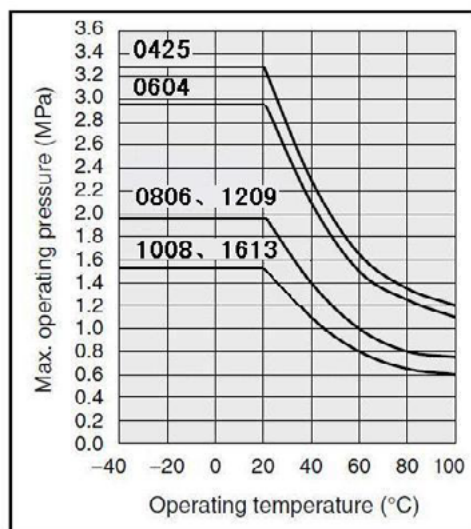
最大操作压力曲线 Maximum operating pressure curve
