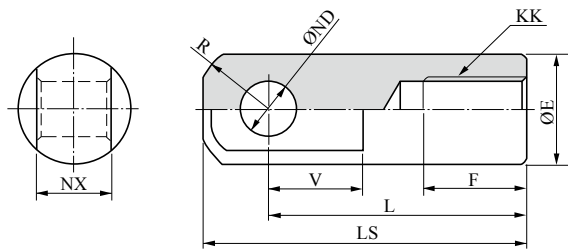
I型单肘节接头 (I Type Single Knuckle Joint)
