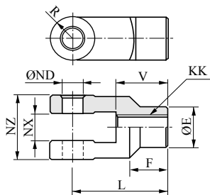
Y型双肘节接头 (Y Type Double Knuckle Joint)
