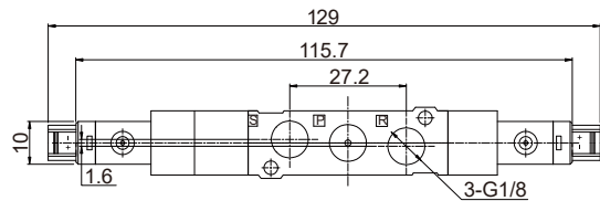
汇流板 Manifold
