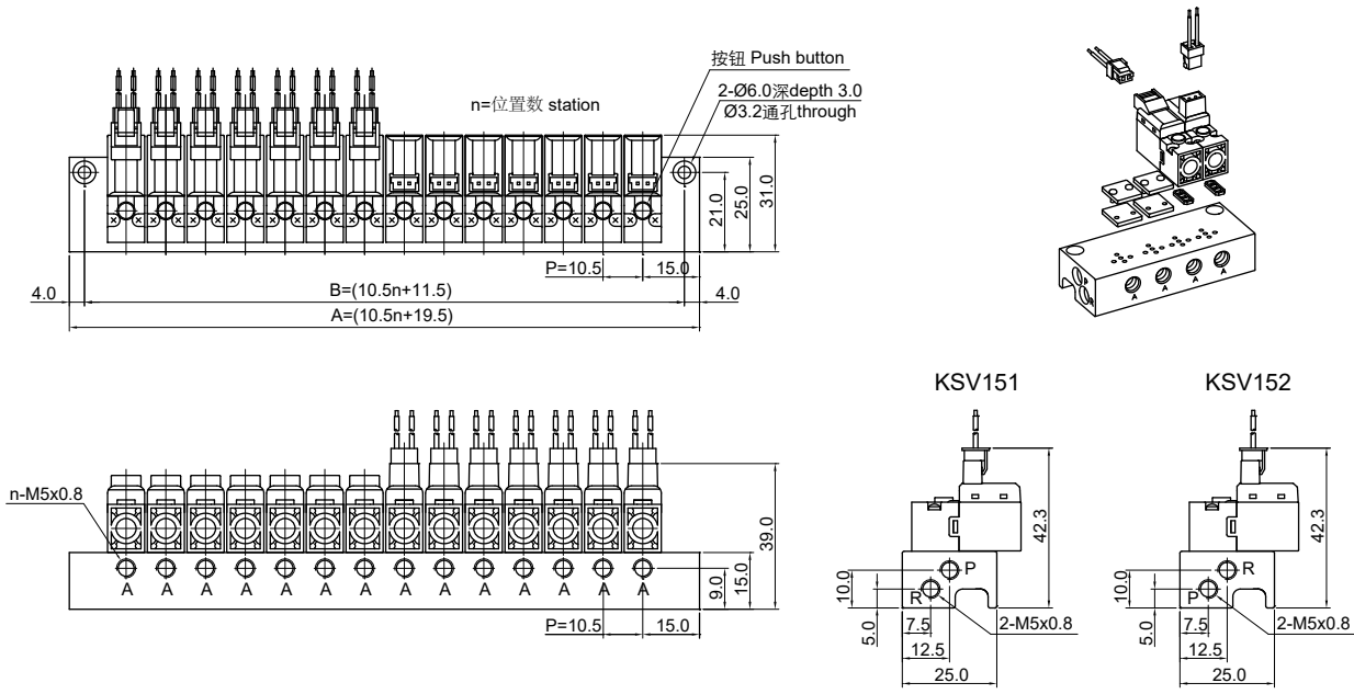
汇流板 Manifold
