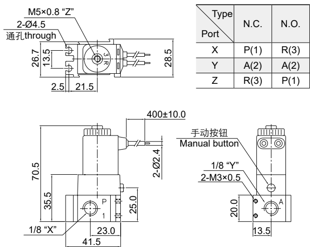
KSV111-G/KSV112-G
