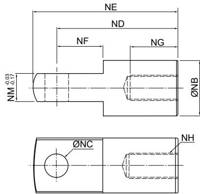
I型单肘节接头 I type single kunckle joint
