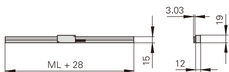
LIC 4113
