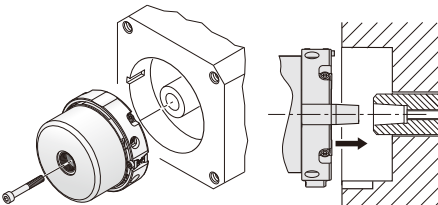
ECN/EQN/ERN 1300
