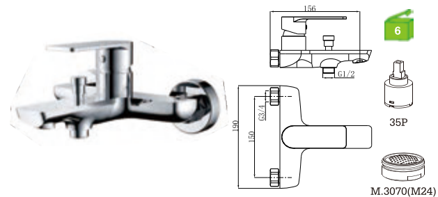
E22BH2C Monocomando banheira Bath/shower mixer Monomando baño
