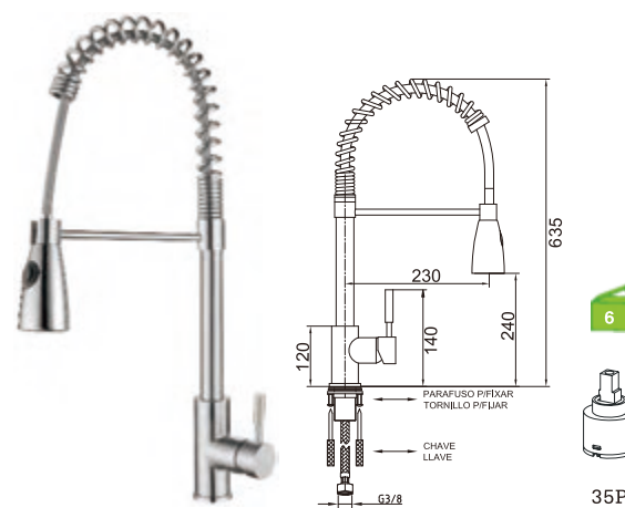
S30LN37X Monocomando de lava-loiça industrial Industry kitchen mixer Monomando de fregadero industrial
