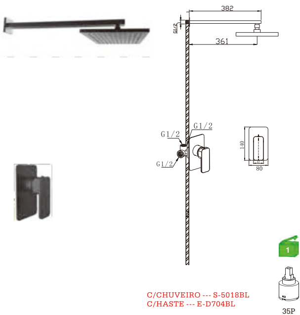
D21RP23BL Monocomando embutido 1 via Built-in mixer Monomando empotrado 1 via 68.30€ (+IVA)
