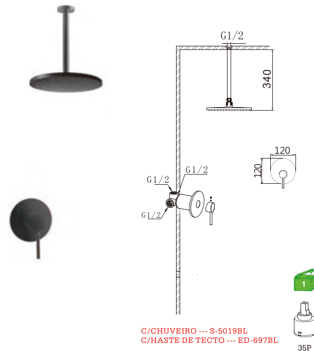
D26FK33BL Monocomando embutido 1 via Built-in mixer Monomando empotrado 1 via 53.50€ (+IVA)
