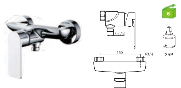
E22BH3C Monocomando duche Shower mixer Monomando ducha
