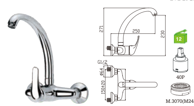
A68M9C Monocomando lava-loiça à parede bica alta Wall mounted kitchen mixer Monomando fregadero pared (caño alto)
