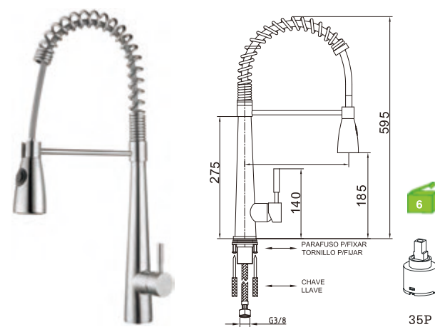
S31LN17X Monocomando de lava-loiça industrial Industry kitchen mixer Monomando de fregadero industrial
