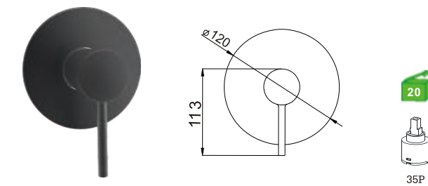
D26FK13BL(B) Monocomando embutido 1 via Built-in mixer Monomando empotrado 1 via 36.30€ (+IVA)
