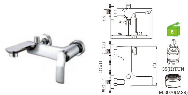
E38BS2C Monocomando banheira Bath/shower mixer Monomando baño
