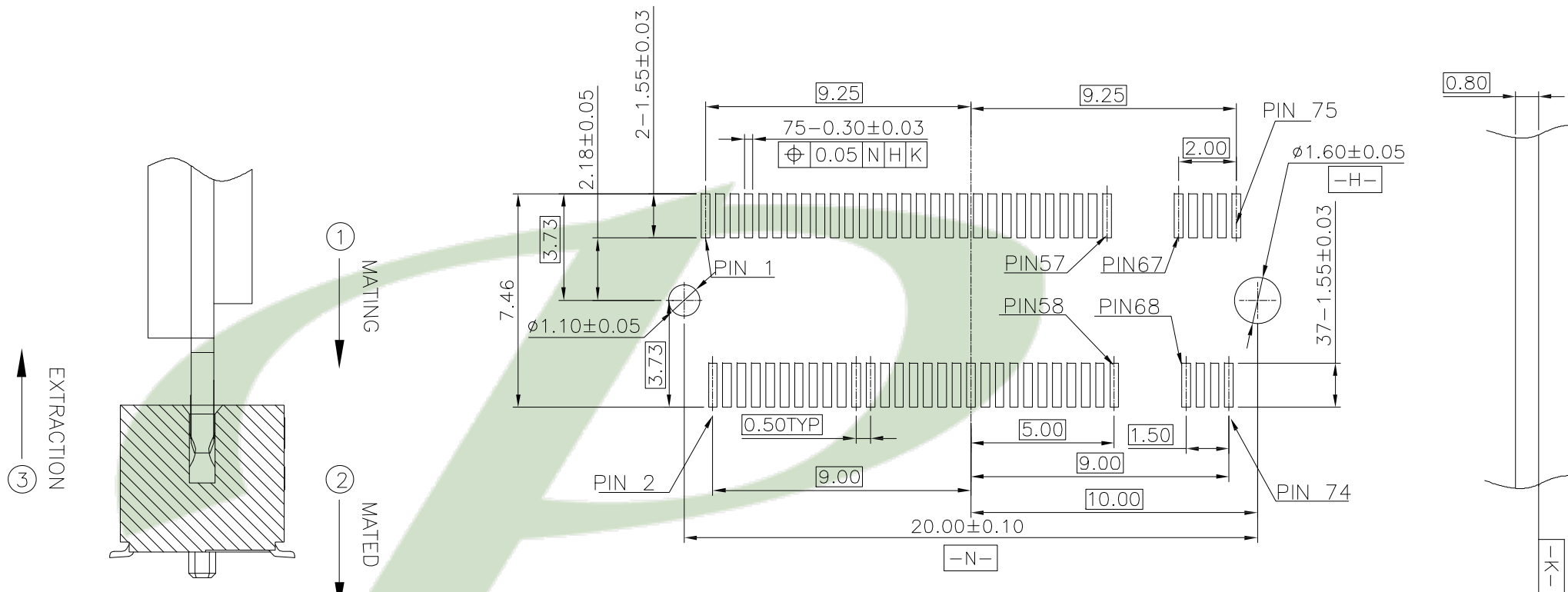
RECOMMENDED PCB LAYOUT(TOP VIEW) DEFAULT TOLERANCE ±0.05MM
